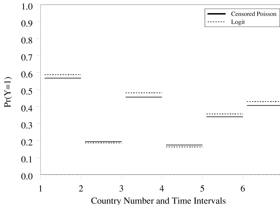
Fig. 3 Time-independent data ( \beta_0 = -3 , \beta_1 = 2 ): probability of event occurrence for the censored-poisson and logit models. The figure shows the predicted censored-poisson and logit probabilities of an event occurring for a sample of six countries over 10 time subintervals in each country. Each country is denoted by the number on the x axis, with its 10 time subintervals following. The probability of an event occurrence is calculated for each subinterval using the country-varying data X_c and the censored-poisson and logit regression estimates obtained from the larger data set. The figure shows that for time-independent data, the logit model predicts similarly to the censored-poisson model. Note, however, that, unlike the censored-poisson estimates, the logit estimates will not be directly comparable to the exponential and poisson estimates.
