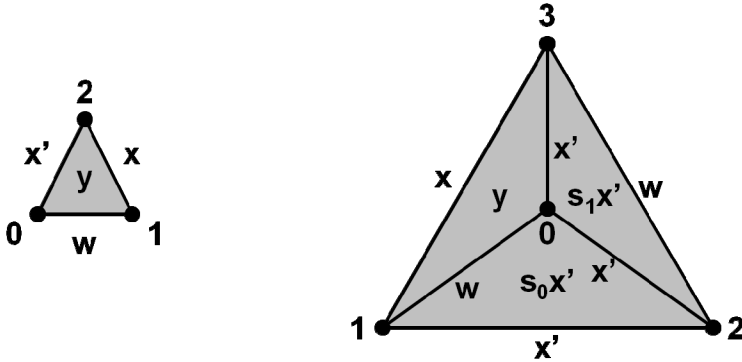
FIGURE 28. Shifting indices in the homotopy relation. Here w stands for d_2 s_0 x = d_2 s_0 x' , which is a degenerate 1-simplex, both vertices being the first vertex of x , which is also the first vertex of x' .
