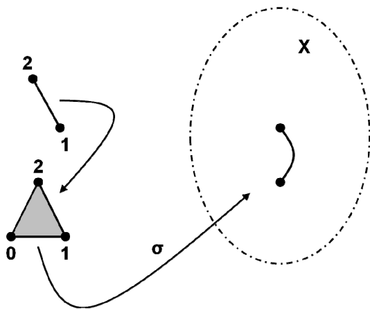
FIGURE 14. A face of a singular simplex.
