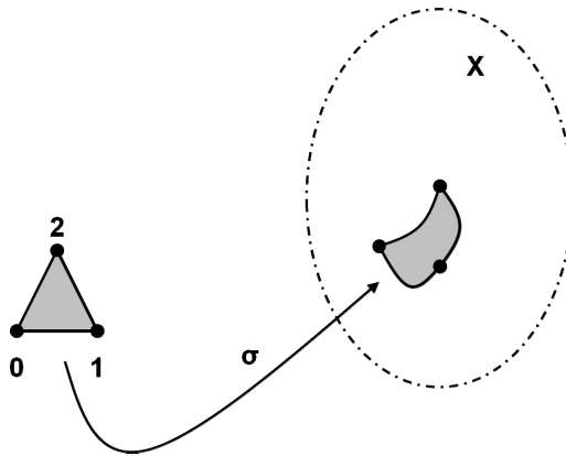
FIGURE 13. A singular simplex.
