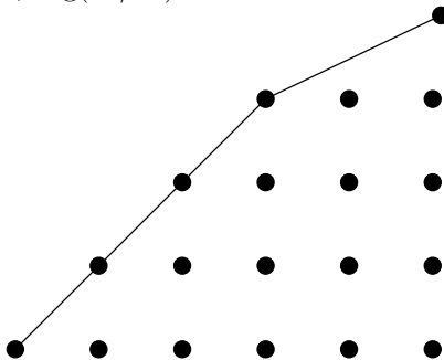
FIGURE 1. The HN polygon associated to an object V admitting a filtration 0 = V_0 \subset V_1 \subset V_2 = V with \text{rank}(V_1) = 3 , \text{deg}(V_1) = 3 , \text{rank}(V_2/V_1) = 2 , \text{deg}(V_2/V_1) = 1 .
