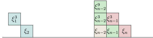
Figure 5-1: Illustration of the decomposition of B_n into tensor factors
