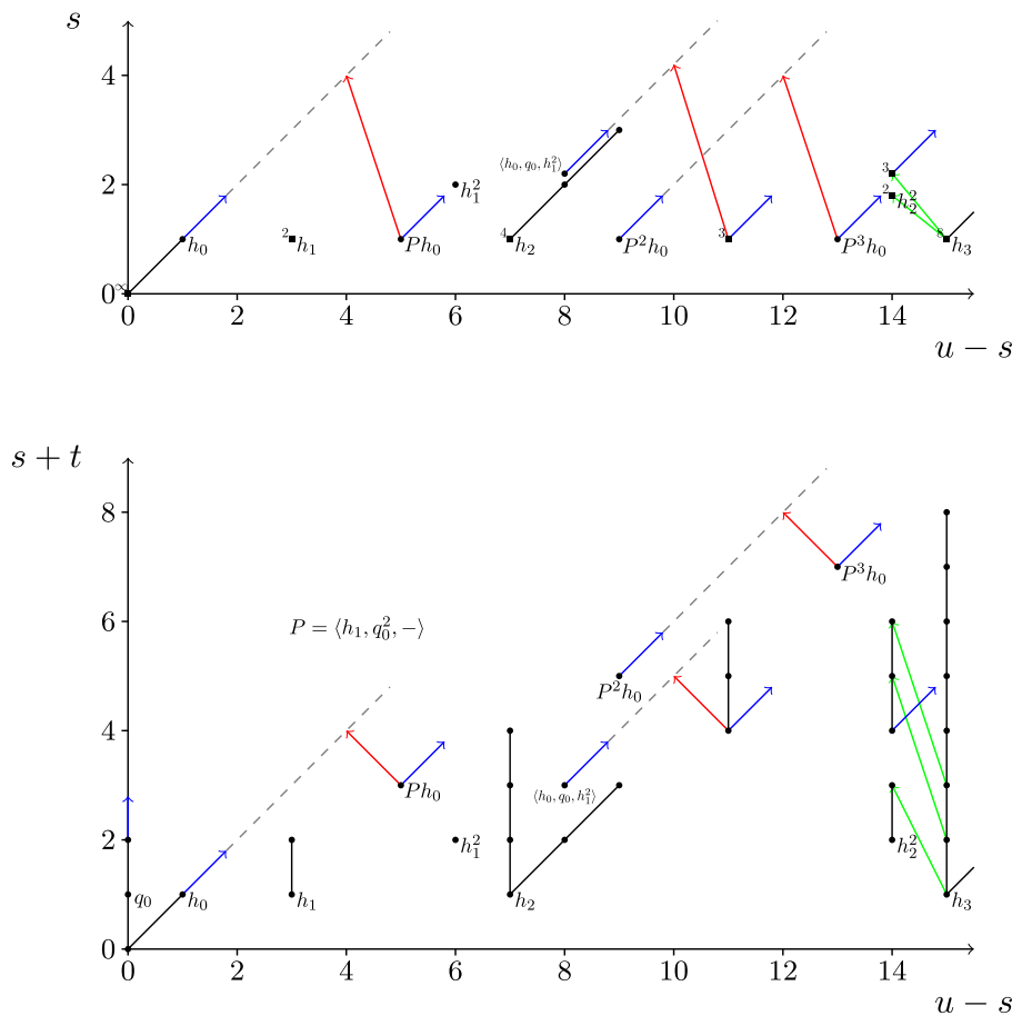
FIGURE 1 (colour online). H^*(P; Q) in Novikov and classical Adams projections. Green arrows are algebraic Novikov differentials and red arrows are Cartan–Eilenberg differentials.
