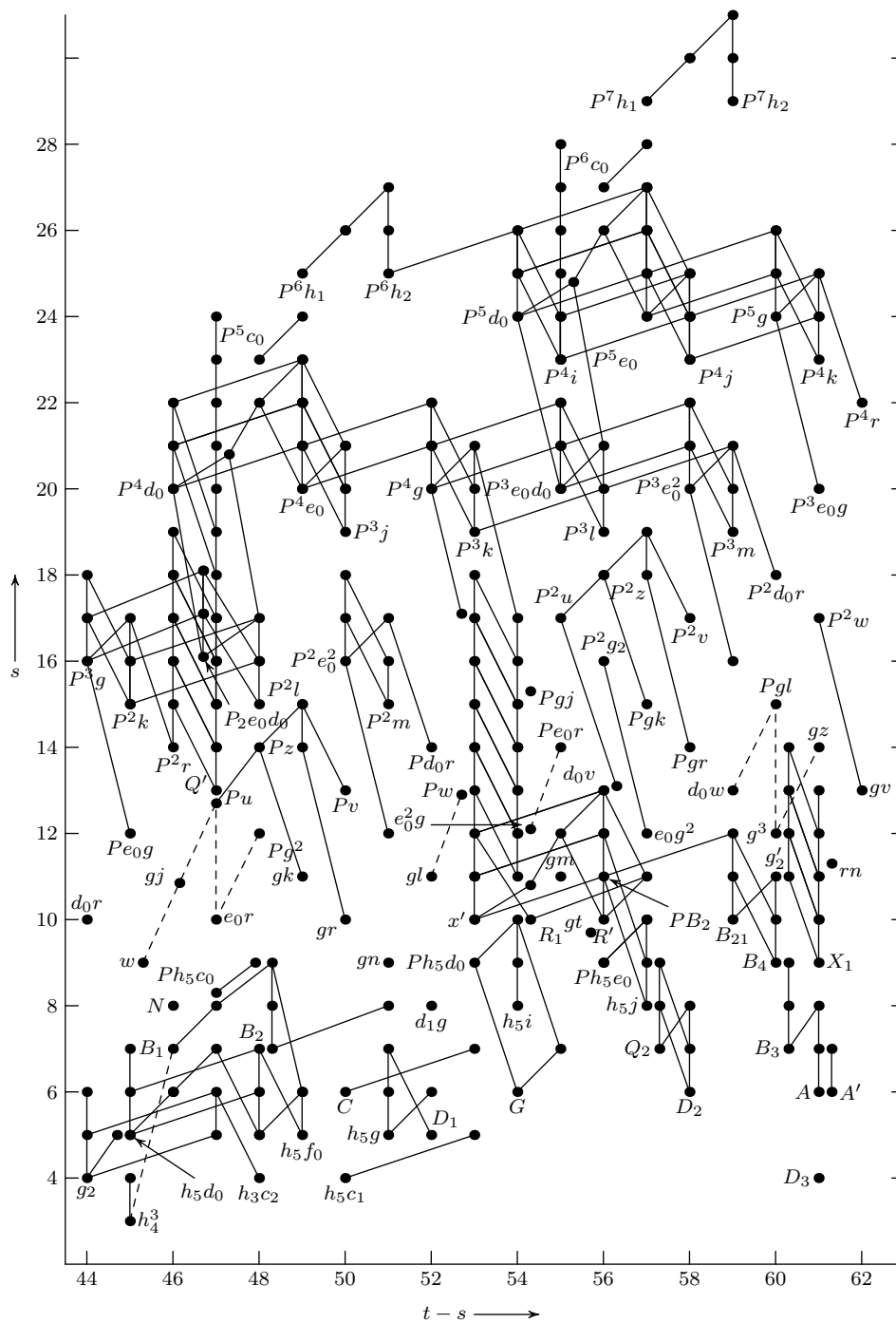
FIGURE A3.1c. The Adams spectral sequence for p = 2 , 44 \leq t - s \leq 61 . Differentials are tentative, see Isaksen [2] for a better chart.
