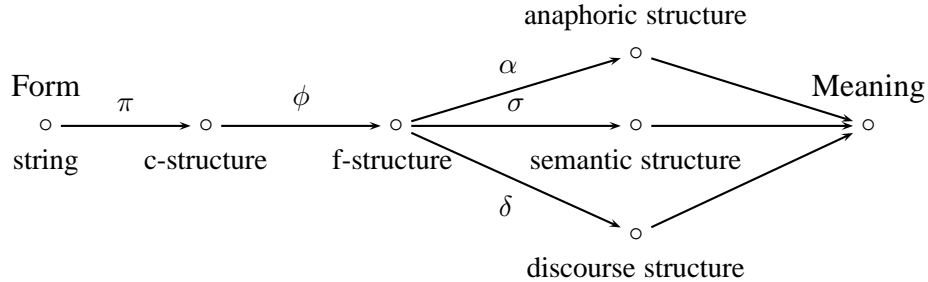
Figure 2.2: An early version of LFG's projection architecture
