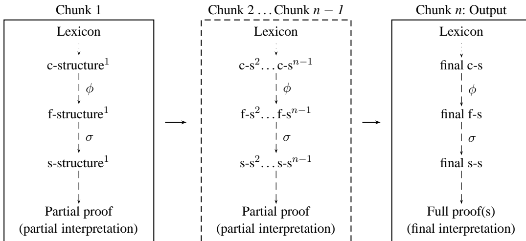
Figure 8.2: The parsing model
