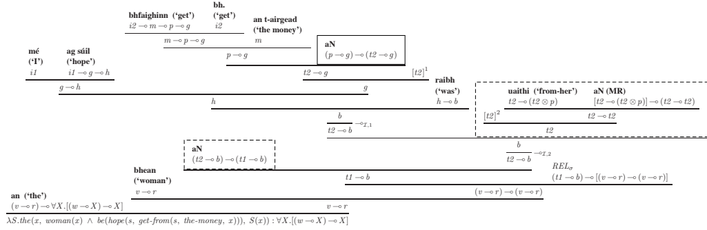
Figure 6.3: Irish Pattern 3 proof
