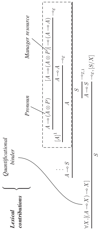
Figure 5.3: A manager resource in action (quantificational binder)
