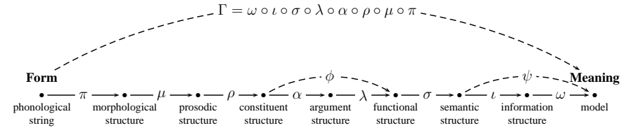
Figure 1: The Correspondence Architecture, pipeline version (Asudeh 2011a)
