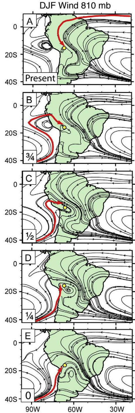
Fig. 4. Simulated austral summer 810-mb wind streamlines for modern (A), \frac{3}{4} (B), \frac{1}{2} (C), \frac{1}{4} (D), and no-Andes (E) cases. All data represent 5-year December–January–February (DJF) averages of RegCM simulations. Flow onto the central Andean Plateau (yellow filled circle) is denoted by a thick red line. The summer wind direction changes from predominantly westerly (B–E) to northeasterly (A) as plateau elevations are increased. The shift in wind direction would influence the source and fractionation history of vapor precipitated over the plateau.
