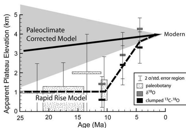
Fig. 6. Paleoclimate influence on apparent paleoelevation reconstructions from the central Andean Plateau. Previously published paleoaltimetry proxies used to suggest a rapid rise of plateau (thick dashed line) are shown with 1- and 2-sigma uncertainties (Gregory-Wodzicki et al., 1998; Gregory-Wodzicki, 2000; Garzzone et al., 2006; Ghosh et al., 2006). On the basis of our climate model results, we estimate a >0.3 – 4.5 km paleoclimate correction should be applied to the paleoaltimetry data. The gray shading represents our estimated range of possible plateau elevations after application of a paleoclimate correction to the rapid-rise model. The solid line represents our estimated average elevation history after correction. See Section 5.4 for details.
